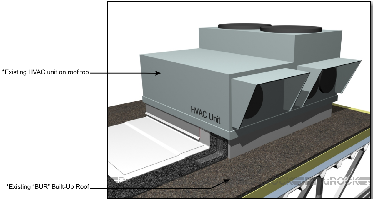
SYSTEM APPLICATION AROUND HVAC UNIT (VIEW A)
