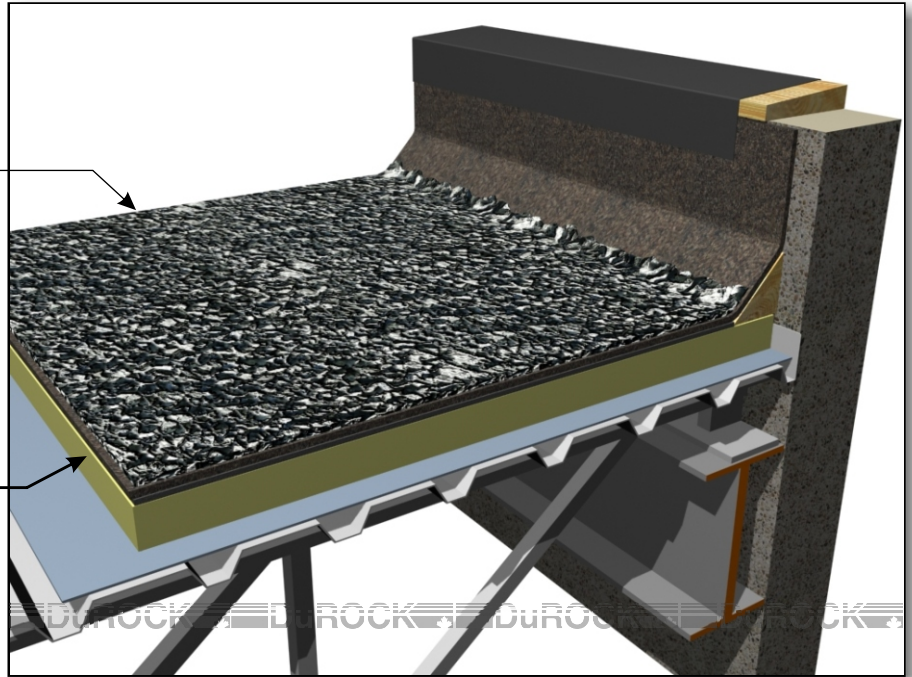
BUILT-UP ROOF BEFORE SYSTEM APPLICATION
