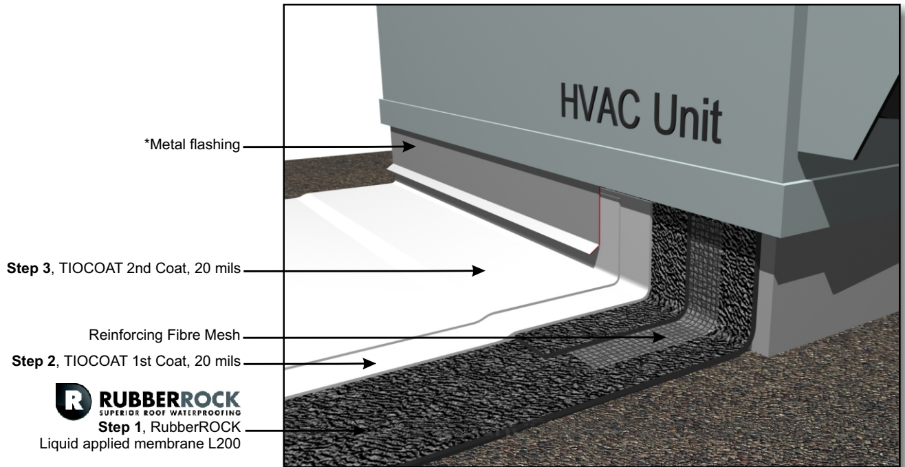
SYSTEM APPLICATION AROUND HVAC UNIT (VIEW B)
