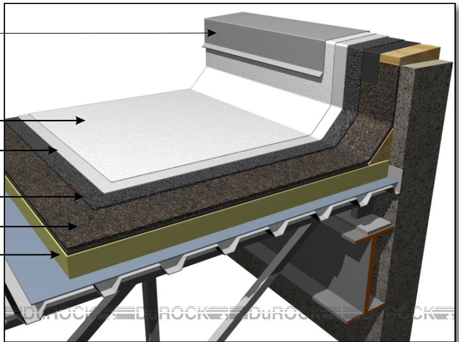
BUILT-UP ROOF AFTER SYSTEM APPLICATION
